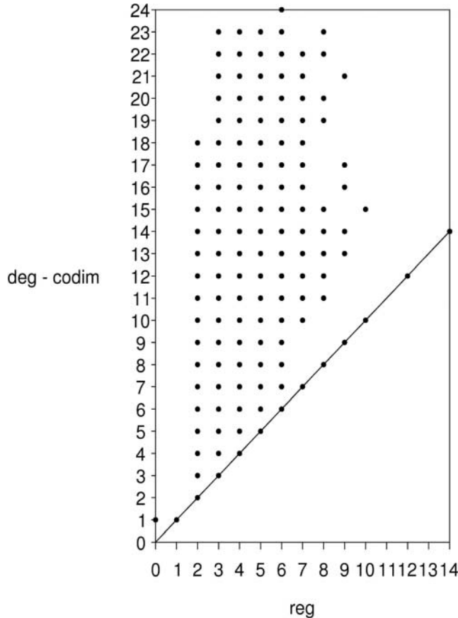
FIGURE 1. \text{deg } \mathbb{Q}[B] - \text{codim } \mathbb{Q}[B] against \text{reg } \mathbb{Q}[B] for \alpha = 3 and d = 4 .
