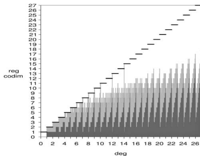
FIGURE 2. \text{reg } \mathbb{Q}[B] + \text{codim } \mathbb{Q}[B] against \text{deg } \mathbb{Q}[B] for \alpha = 3 and d = 4 .
